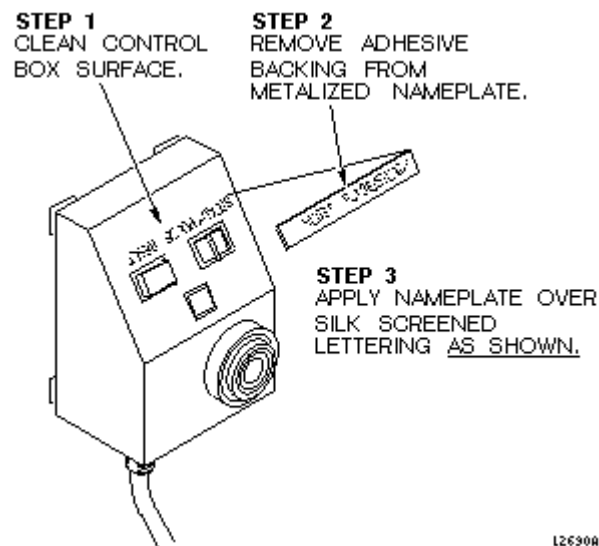
NAME PLATE APPLICATION ILLUSTRATION 2-1
